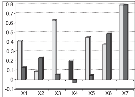
Figure 2: Simple correlation coefficients and direct effects of the seven yield components of seed yield.
