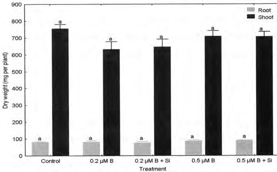
Figure 1: Effect of Si on root and shoot dry weight of sunflower plants subjected to low B external supply (0.2 \mu\text{M} B and 0.5 \mu\text{M} B). Si concentration in nutrient solution was 1.5 mM. Data are means ( n=4 ) \pm SD. Significant differences at p\leq 0.05 are indicated by different letters.
