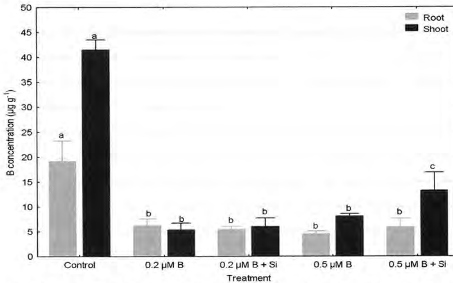
Figure 2: Effect of Si on B concentration in roots and shoots of sunflower plants subjected to low B external supply (0.2 \mu\text{M} B and 0.5 \mu\text{M} B). Si concentration in nutrient solution was 1.5 mM. Data are means ( n=4 ) \pm SD. Significant differences at P\leq 0.05 are indicated by different letters.
